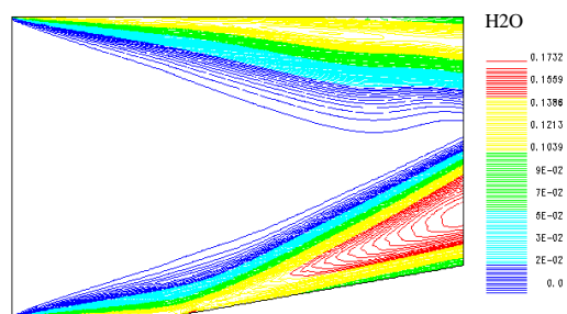
Figure G4.9 Contour lines of H 2 O concentration for flow past a ramped duct.
