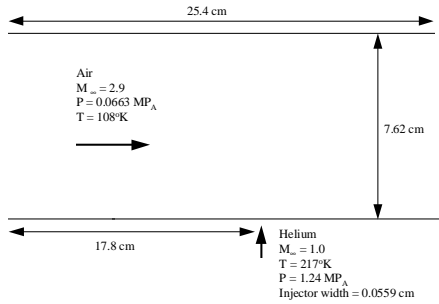
Figure G3.1 Computational domain for the transverse injection of Helium into an air stream.
